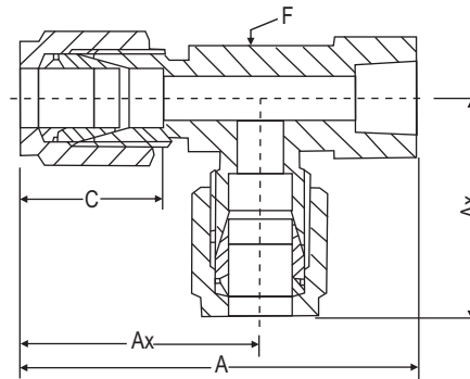
Dimensional Details :
